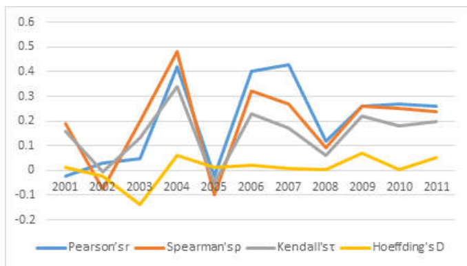
Figure 15. Annual variations in correlation coefficients according to the different tests
